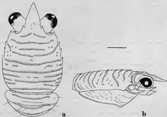
FIG. 1. — Alaius crossneri sp. nov., ♀ holotype from Stn DW 471 (MUSORSTOM 6) : a, carapace and abdomen, dorsal view; b, carapace, lateral view.
